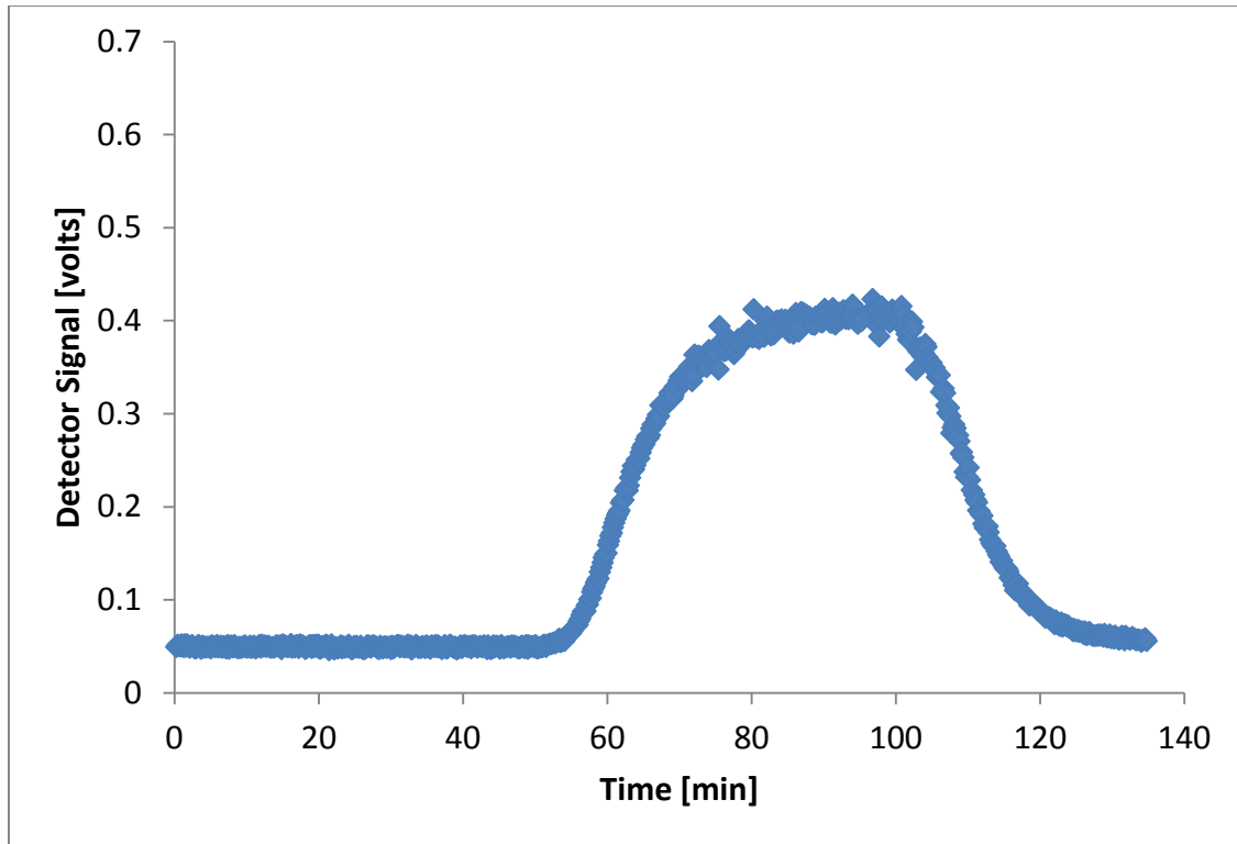
Figure 6.6. Chromatogram of 50 mg/mL S-ibuprofen 40°C and 150 Bar FACP
