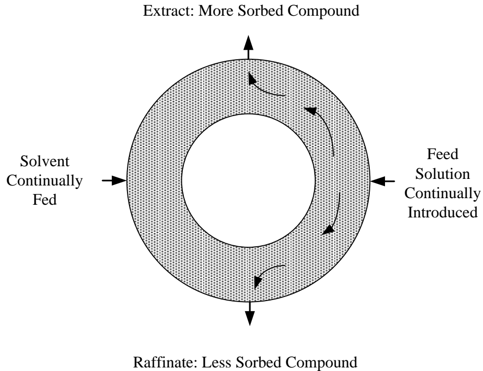
Figure 1.10. True Moving Bed Process
