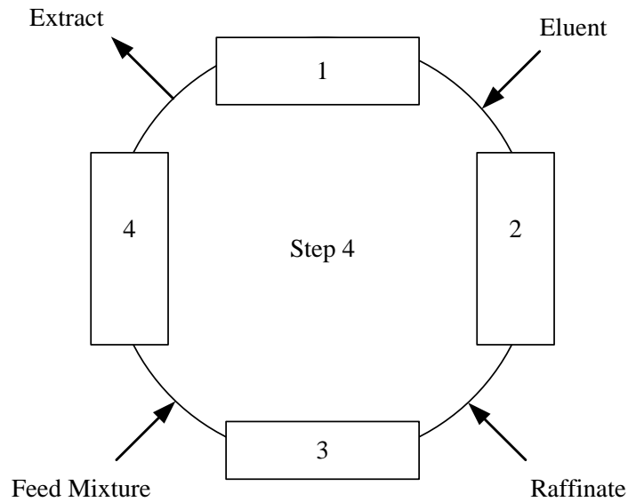
Figure 1.17. Simulated Moving Bed Time Step Four
